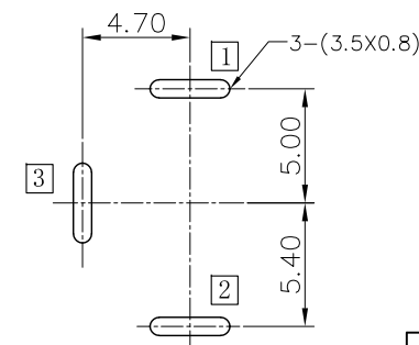
P. C. B Layout (Tolerance: \pm 0.1 ) (Copper-sided view)
