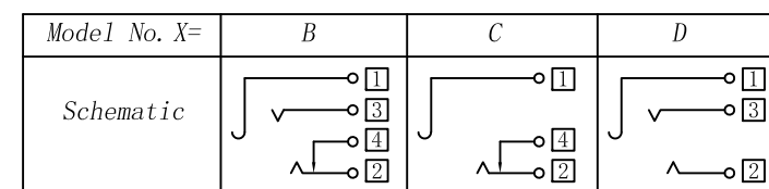
Circuit Diagram □: Terminal No.
