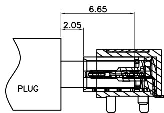
AFTER MATING
