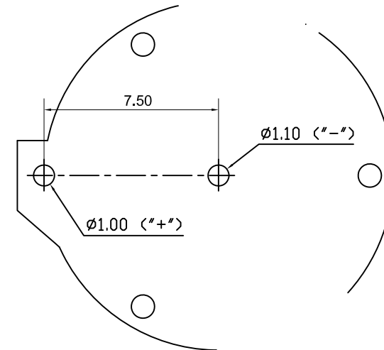
PCB LAYOUT
